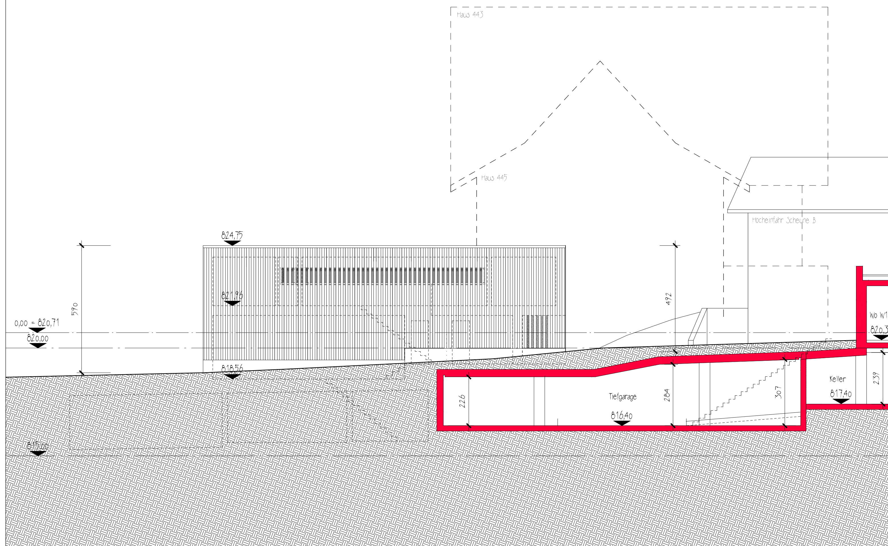
Fassade West
