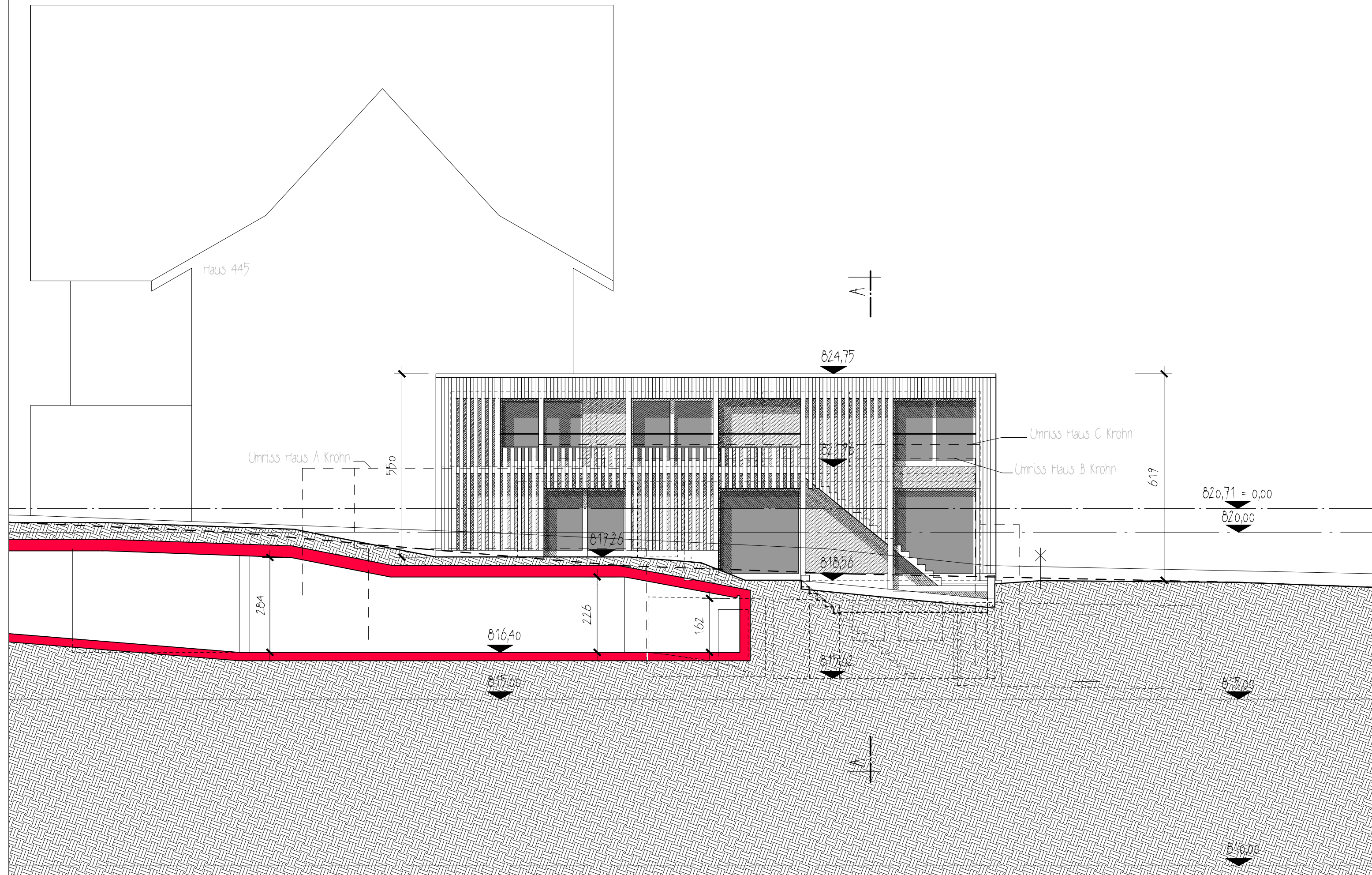
Fassade West
